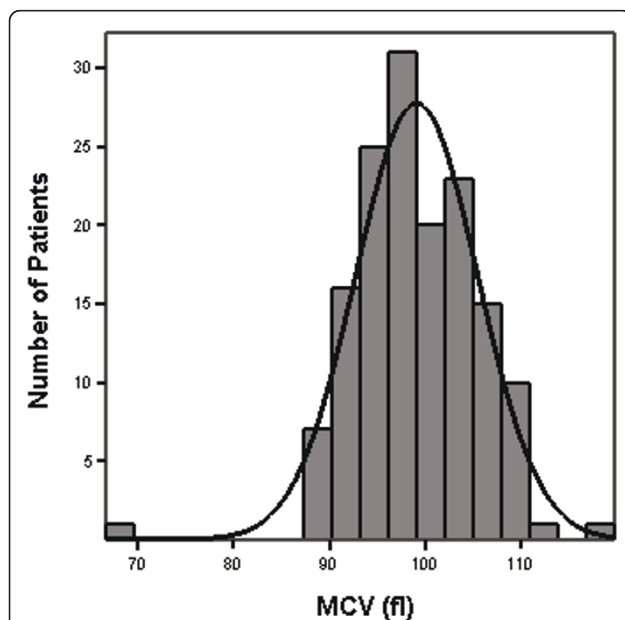
Figure 2 Distribution of MCV (fl). Mean MCV was 99.1 \pm 6.4 fl, (range 66-120 fl).
