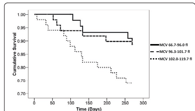
Figure 3 Kaplan Meier survival in tertiles of MCV (fl). Log rank p = 0.047
